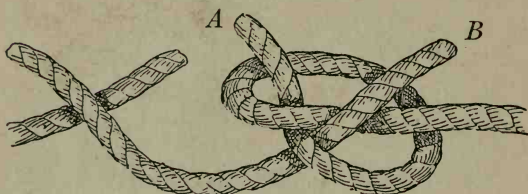
FIG. 23.—Weaver's knot (tying).
